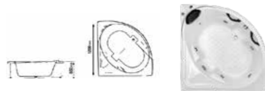
MODEL ARGHAVAN (ارغوان) Size: 1300 * 750 * 460mm
